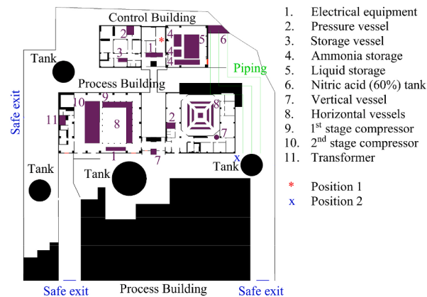
Fig. 14. Map A for on-site simulation purpose.
