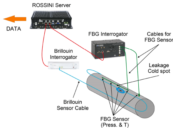
Fig. 2. Schematic of the proposed FO system.
