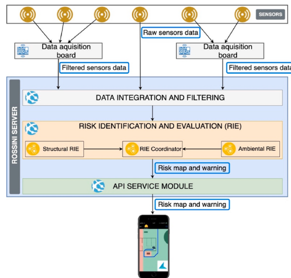
Fig. 9. ROSSINI system architecture.
