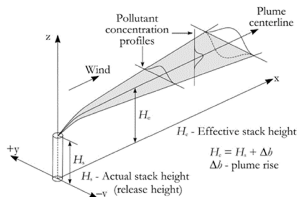
Fig. 8. Diffusion of pollutants from a point source [48].
