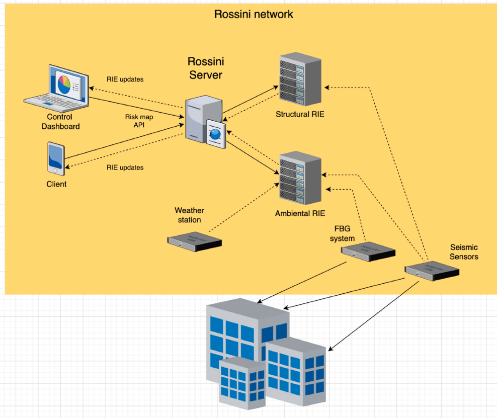
Fig. 4. Illustration of sensors and their interaction within the RIE modules.
