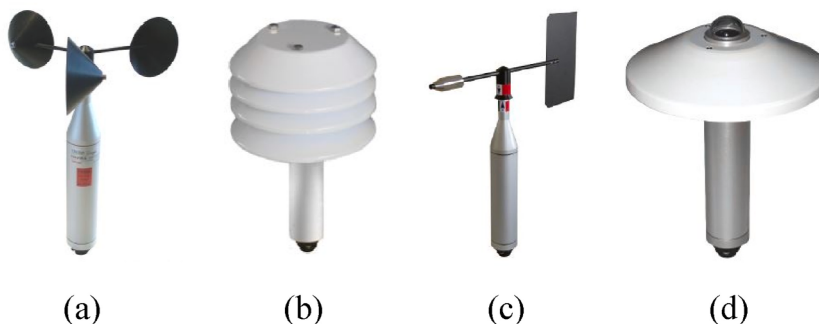
Fig. 3. Weather station comprising of (a) wind speed sensor; (b) thermogravimetric sensor; (c) wind direction sensor; and (d) solar radiation sensor.
