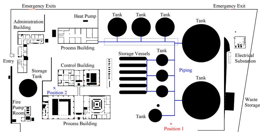
Fig. 15. Map B for simulation purposes in a virtual environment.
