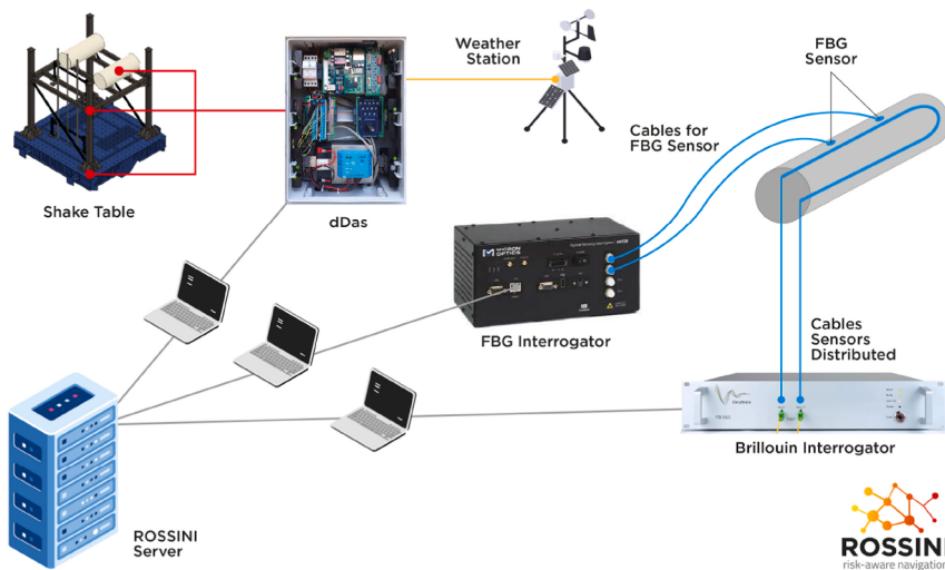
Fig. 17. Sensors' layout and connection to ROSSINI server.
