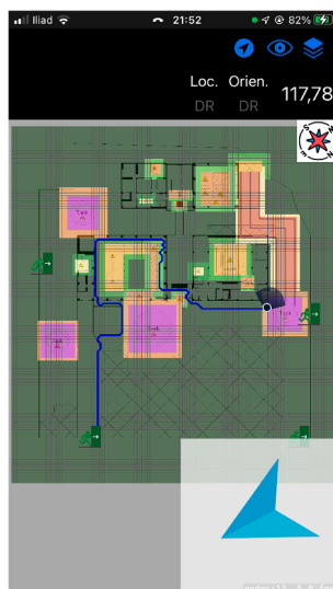
Fig. 13. Example illustration of how the navigation system takes the industrial plant worker along the safest path and not necessarily the closest.
