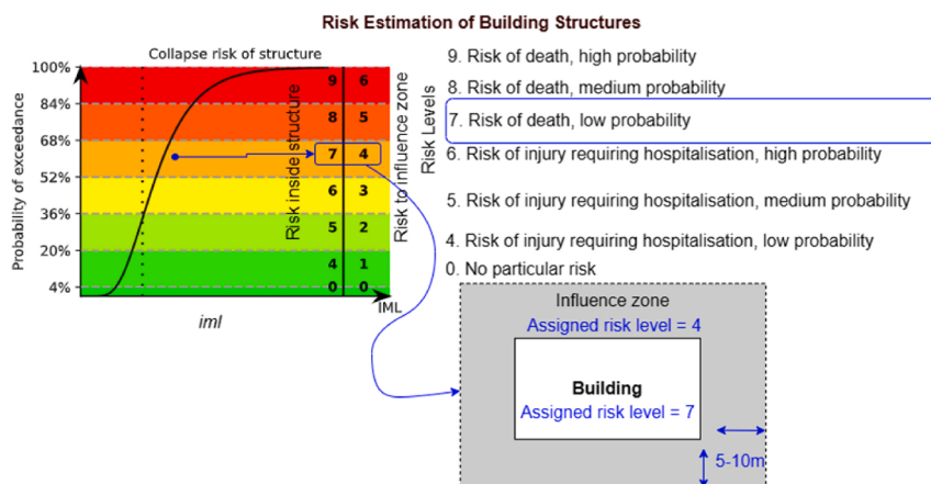
Fig. 7. Estimation of structural risk metrics inside and outside (influence zone) of a hypothetical building.
