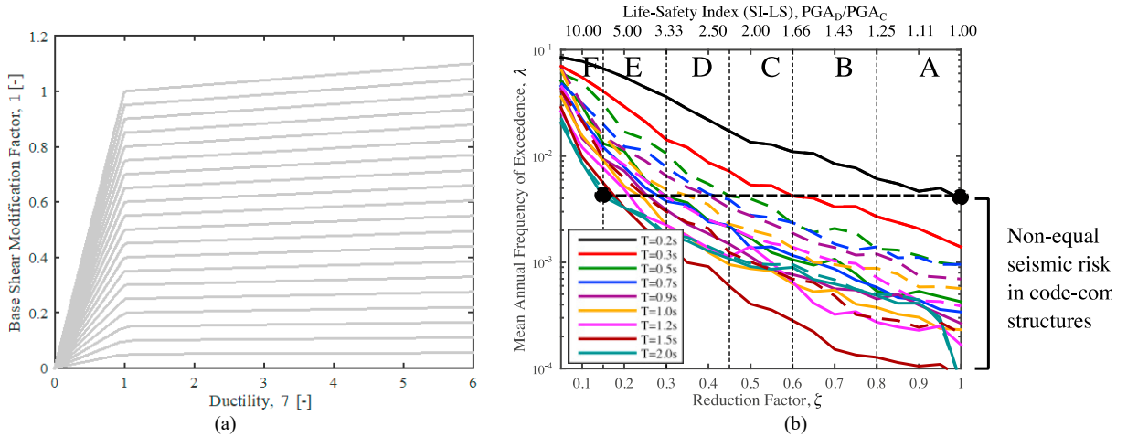
Fig. 3. (a) Example of SDOF oscillators ( T=0.3s and q=3.90 ) illustrating the degradation in lateral strength with respect to the code-compliant value for the design base shear; (b) non-uniformity of risk for SDOFs for both medium (solid lines) and high (dashed lines) ductility classes versus periods of oscillation, T , and strength modification factor, \zeta .
