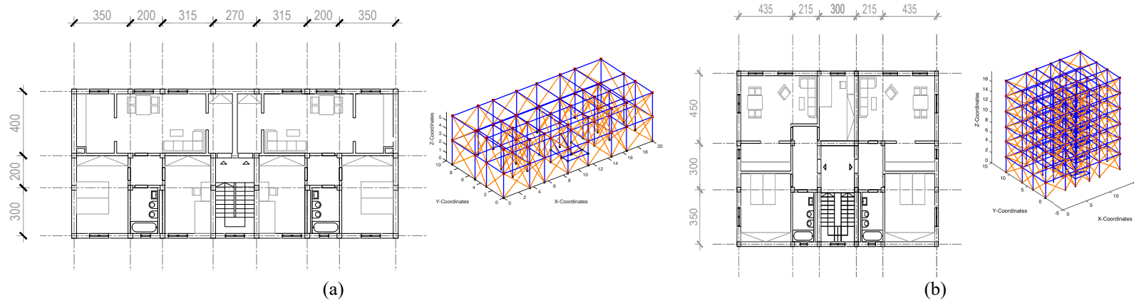
Figure 7. Architectural plan layout and OpenSees numerical model of (a): 2-storey and (b): 6-storey infilled RC archetype buildings.
